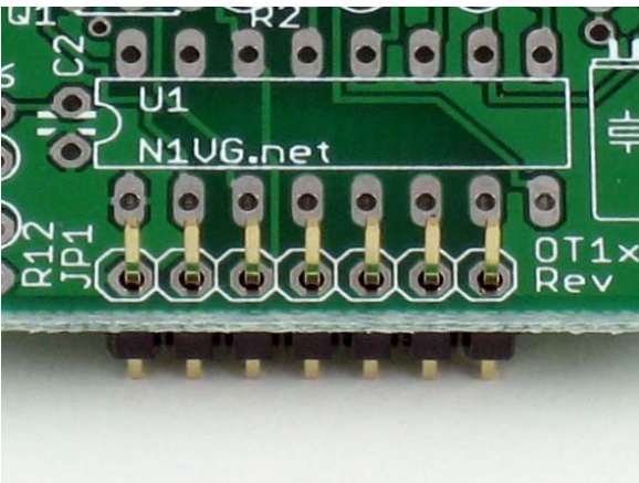
Pin headers installed from the bottom of the board, before soldering.
