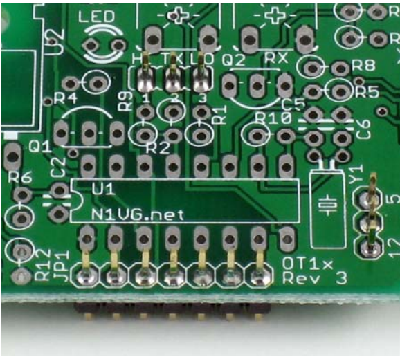
Pin headers after soldering from the top.
